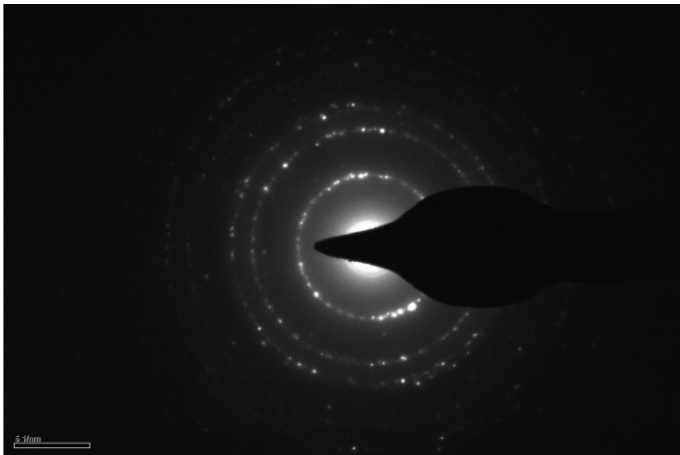
Fig. 8 TEM photo of diamond synthesized by driver tube method
