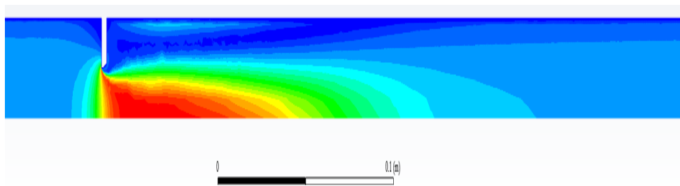
Figure 5 - Velocity contour around the orifice
