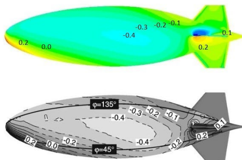
Fig. 16. Validation of distribution of pressure coefficient [24]
