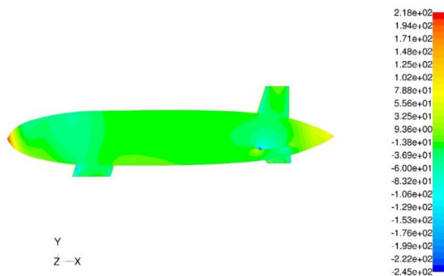
Fig. 6. Pressure coefficient on variant number one in the 5-degree angle of attack
